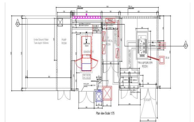
Design of the Technical room
